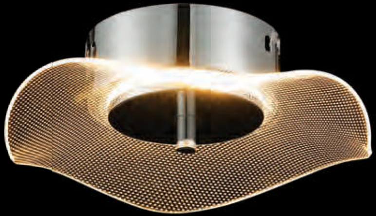
LMT7342 Ø 200 ↓ 200 ↔ 85 (mm) 1 x Integral LED 6W, 460lm Polished Chrome
